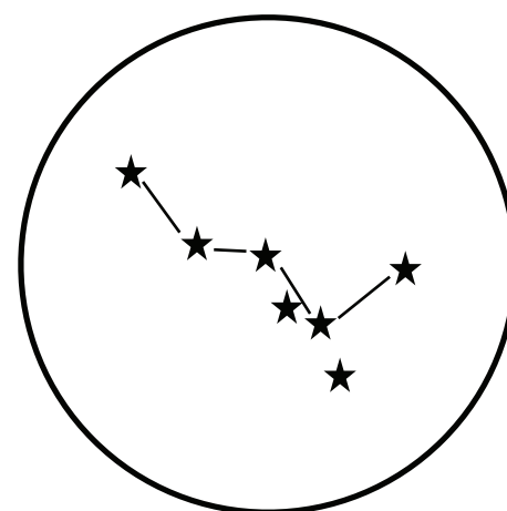
Kaseopeja
